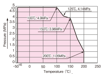
Temperature • Pressure Curve
